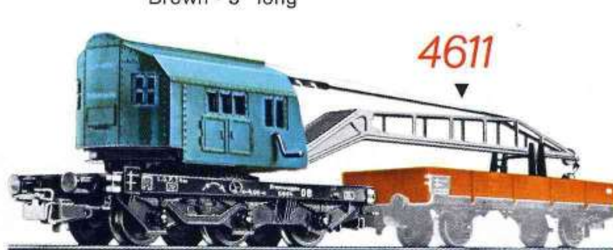
4611 CRANE CAR • With revolving boom and boom adjustment support • Crank handle to raise and lower the crane hook • Black underframe • Blue Cab unit • Silver boom • 3 5/8 in. long • (The 4503 car is not included, but is recommended for supporting the boom when the crane is in transit)
