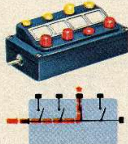
Circuit diagram for 7210 (Switch 3 closed)
