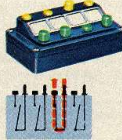
Circuit diagram for 7211 (Switch 3 closed)
