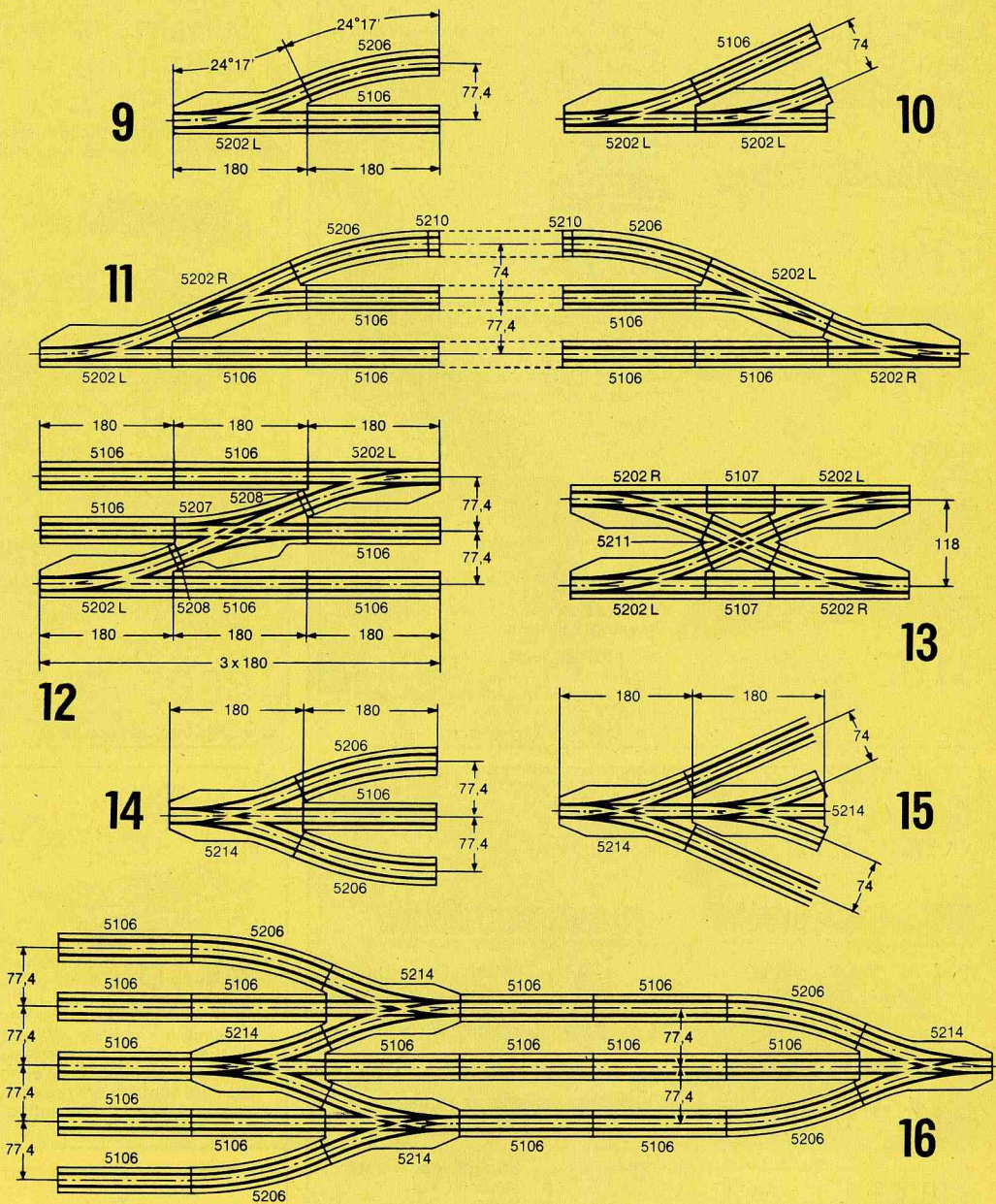
Four solenoid-operated turnouts can be connected to one control box (see page 60).
