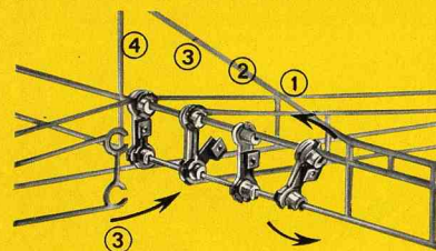
7006 Contact wire insulation · For insu- lating sections of contact wire from cross-spans · One required for each track and cross- span · 15×6 mm ( 5 / 8 "' × 1 / 4 "')
