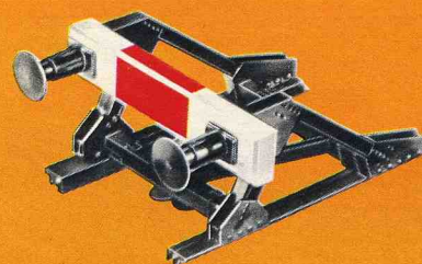
5602 Bumper, riveted steel type · Sprung buffers · Clips onto the rails · Length 98 mm (3 7 / 8 "')
