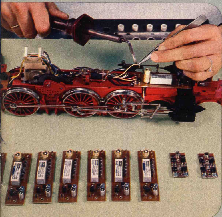
Fitting the electronic direction-control switch in an I-gauge P8 locomotive
