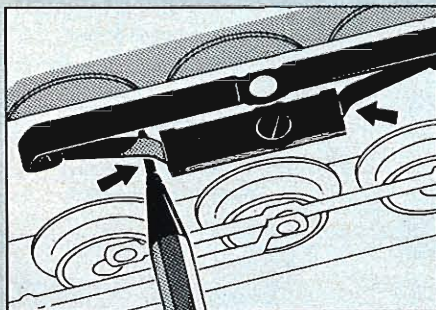
Correcting the pressure of the slider springs
