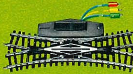
2260 Double slip switch · Radius 424.6 mm (1' 4-3/4") · Operated by electrically by remote control · Can be operated manually also · Tangent length 168.9 mm (6-5/8")
