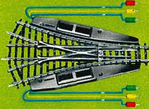
2270 Three-way switch · Operated by 2 double solenoids · Can be operated manually · Both curves symmetrical for multi-track parallel alignment · Tangent 168.9 mm (6-5/8") · Curvature 424.6 mm (1' 4-3/4")
